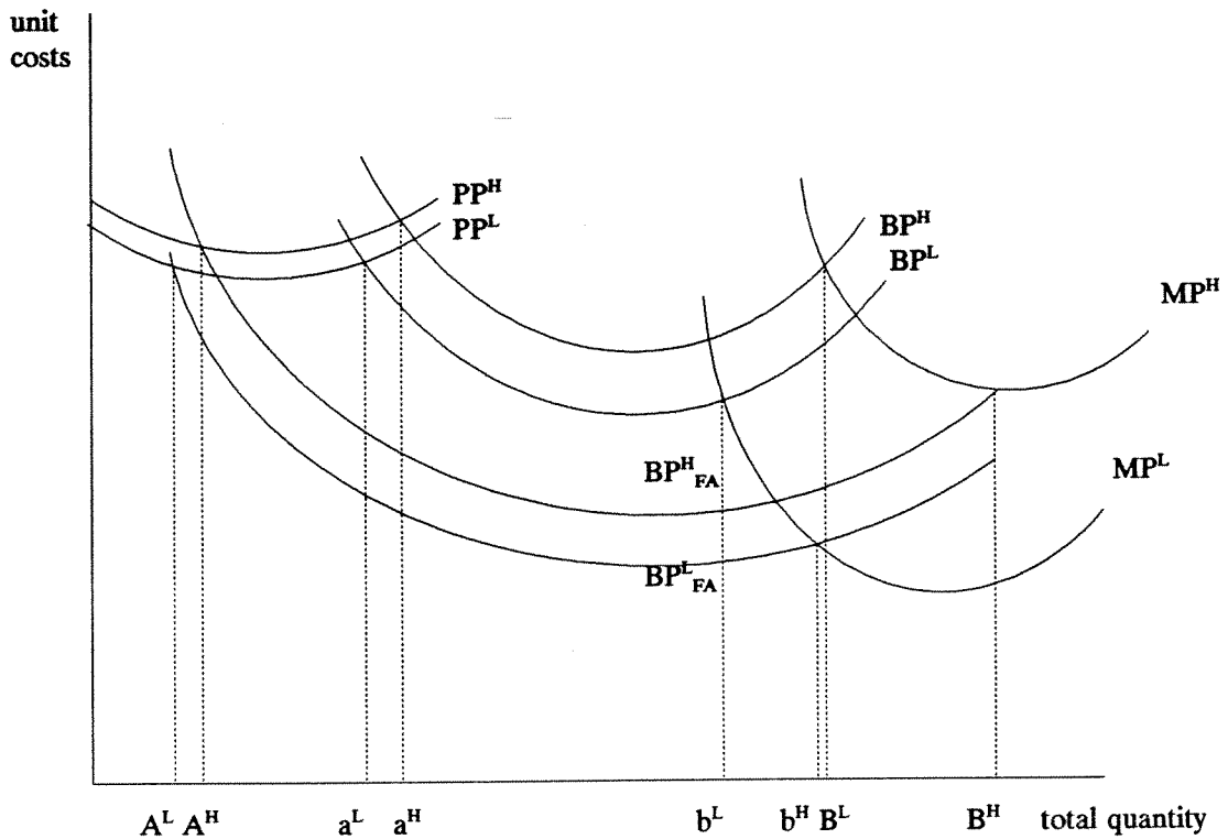
Figure 1 Cost curves of manufacturing systems
