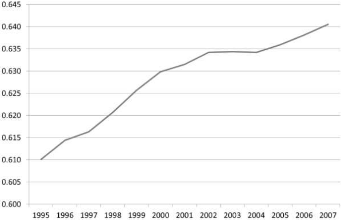
Figure 2. Gini-Coefficient based on Employment in 51 Regions, 1995–2007
