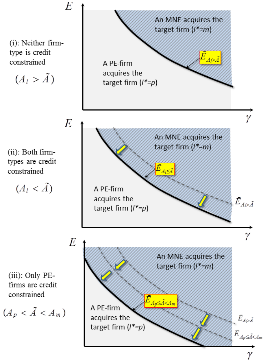
Figure 2: Illustrating Proposition 1
