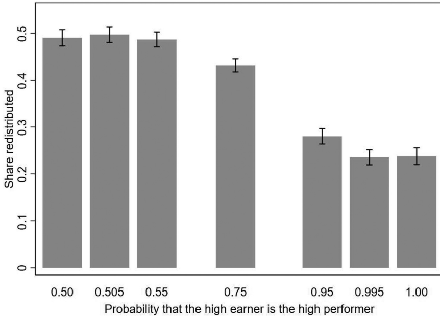
Fig. 2. Share Redistributed for Different Values of p .
