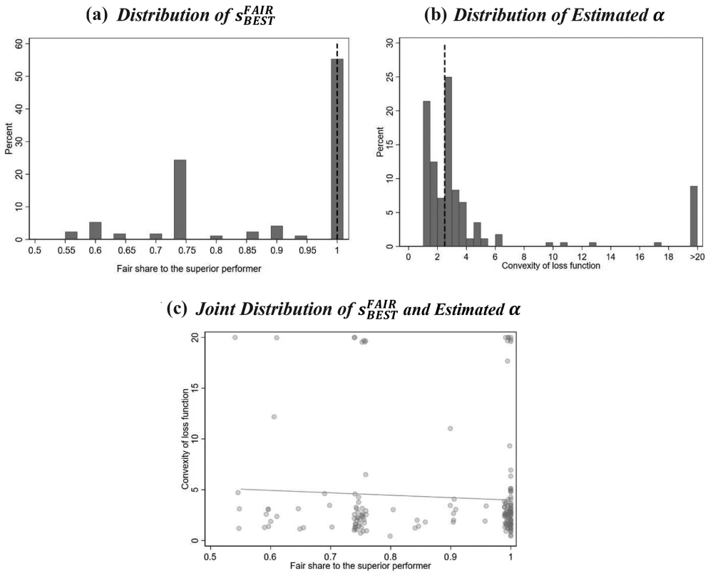
Fig. 3. Individual-level Calibrations for the Meritocrats.
