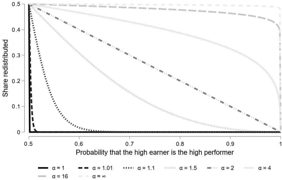
Fig. 1. Predicted Share Redistributed for Meritocrats with Different Values of \alpha .
