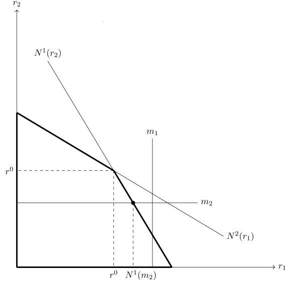
Figure 1: Implementable fees with m_1 > N^1(m_2) > r^0
